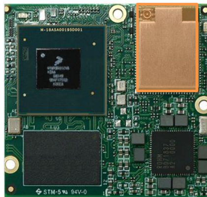
Figure 7 – PICO-IMX8M Wi-Fi Module and Antenna Connector Location
