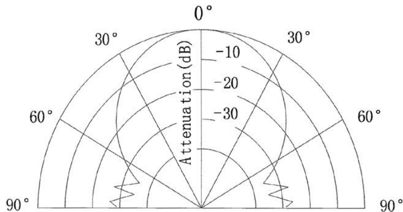
Directivity in Sound Pressure Level
