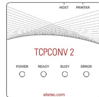
TCPConv 2
