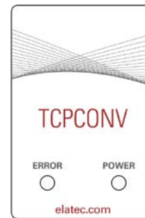
TCPConv
