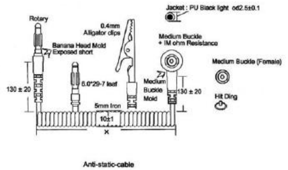
Rotary type electrostatic line 6', 10', 12', 6.5', 12.5', 7' 30AWG*1C Conductor: 7/1250 (1#) Copper wire
