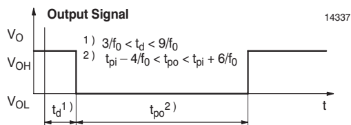
Figure 1. Output Function
