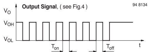
Figure 3. Output Function
