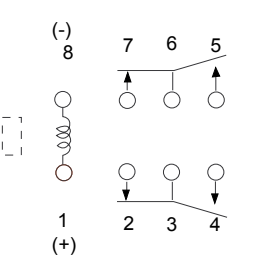
Terminal designations (Top view de-energized position)
