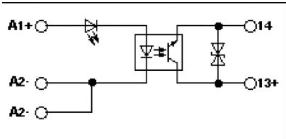
Circuit diagram
