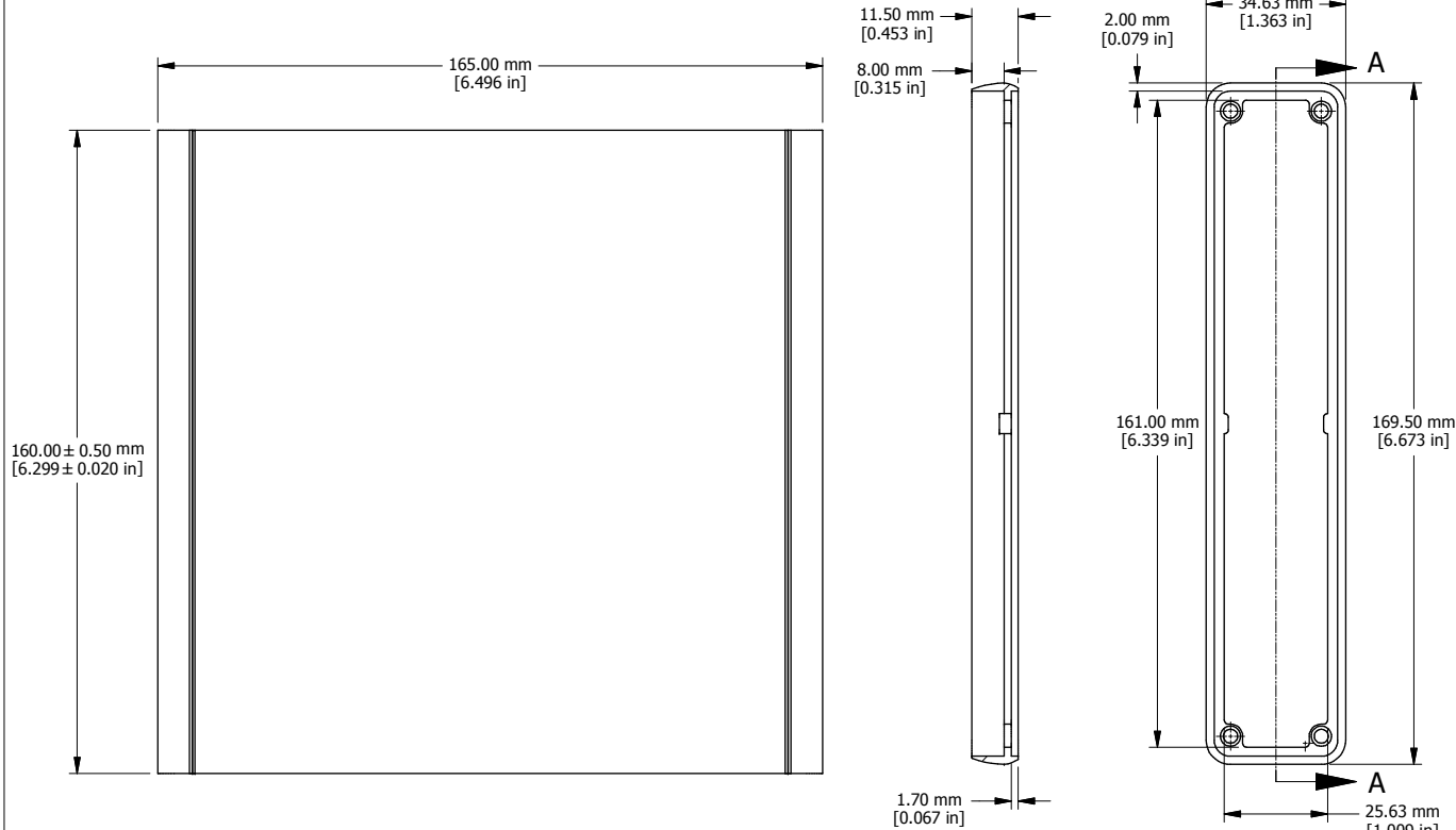
EXTRUSION DESIGNED FOR 160MM WIDE PC BOARD
