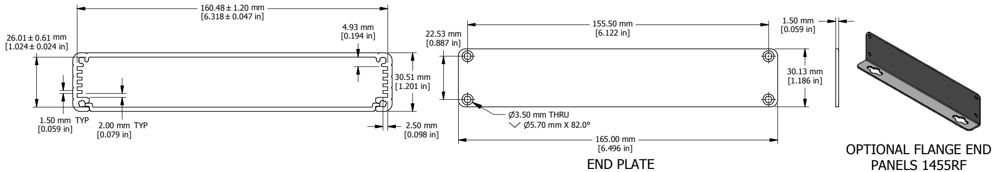
EXTRUSION
