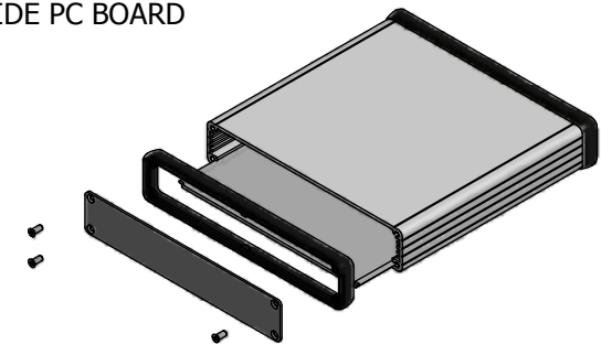
EXPLODED ASSEMBLY VIEW
