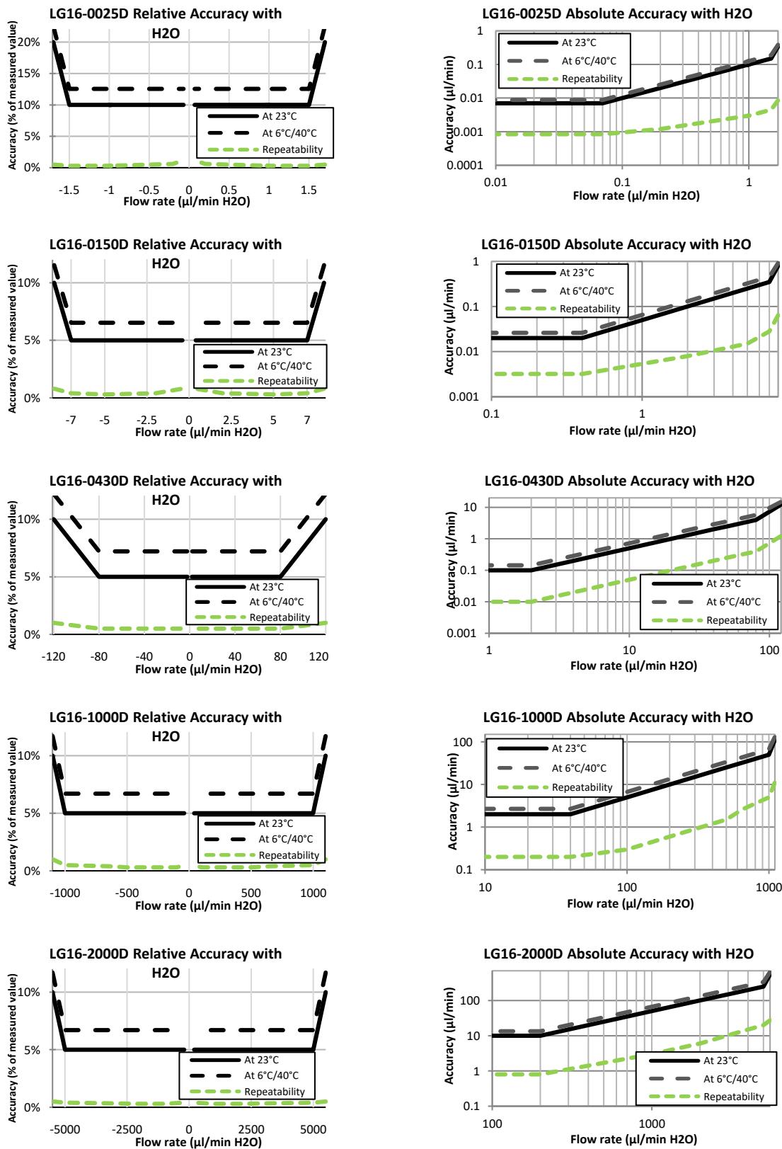
Figure 1: Flow meter accuracy and repeatability across the flow range. Relative error in % of measured value (left column) and absolute error in µl/min (right column) for H 2 O.
