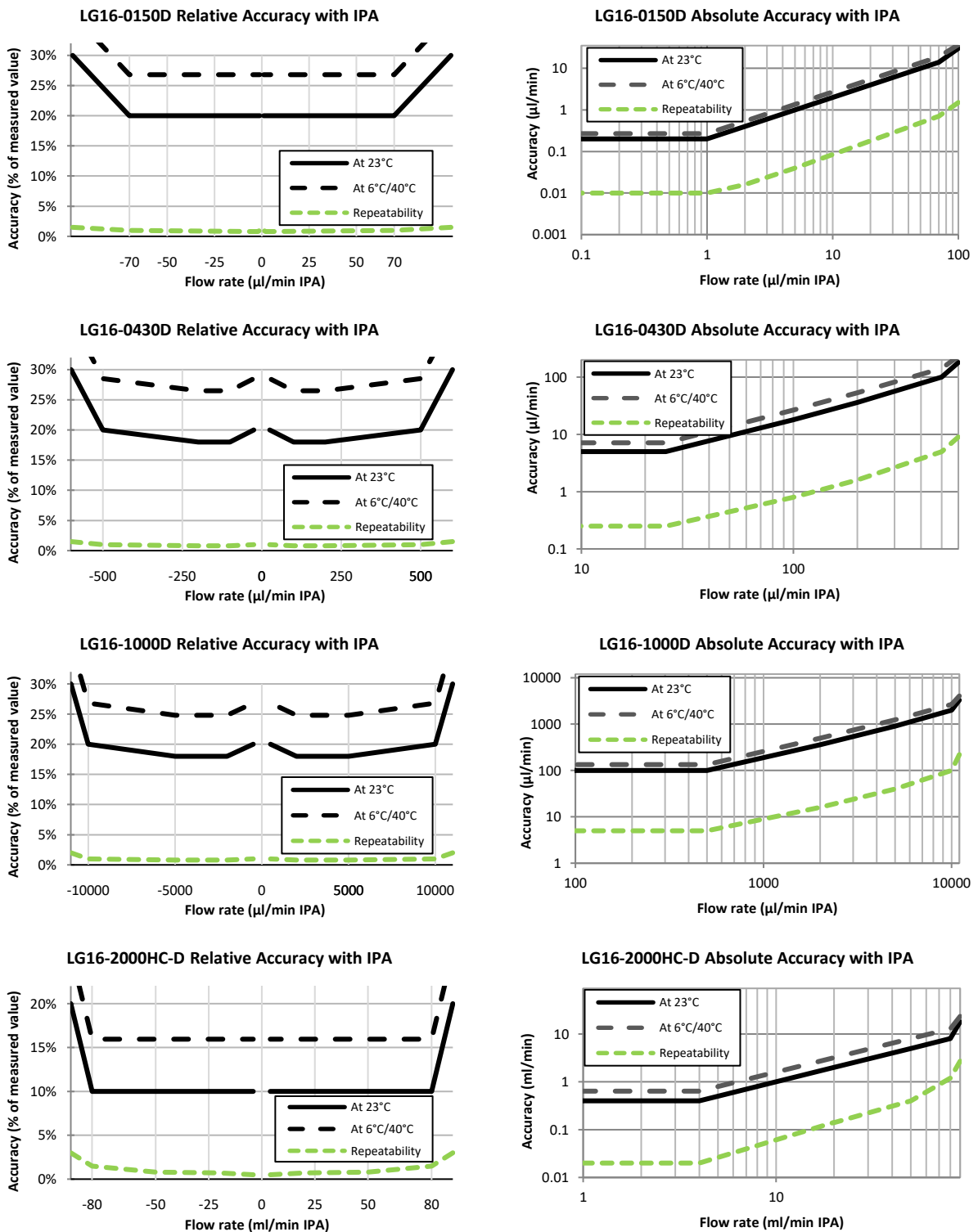
Figure 2: Flow meter accuracy and repeatability across the flow range. Relative error in % of measured value (left column) and absolute error in μl/min or ml/min (LG16-2000HC-D) (right column) for IPA
