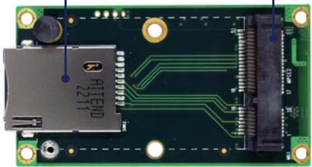
SIM Card Slot (Push-Push) (CU11~CU21) USB 2.0 PIN Header Mini PCIe Full-Size (USB only)
