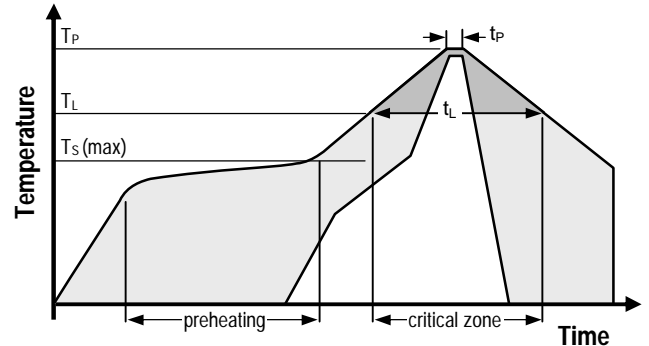
Figure 9 Soldering profile according to JEDEC standard. T_P <= 260^{\circ}\text{C} and t_P < 40\text{sec} for Pb-free assembly. T_L < 220^{\circ}\text{C} and t_L < 150\text{sec} . Ramp-up/down speeds shall be < 5^{\circ}\text{C}/\text{sec} .
