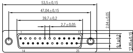
BD25M-DP 9M Mini Adapter(Black Insulator,Nickel Plated)
