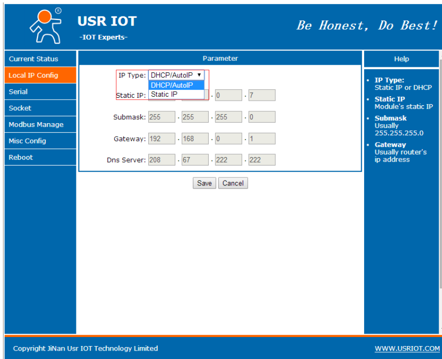
Figure 8 Static IP/DHCP
