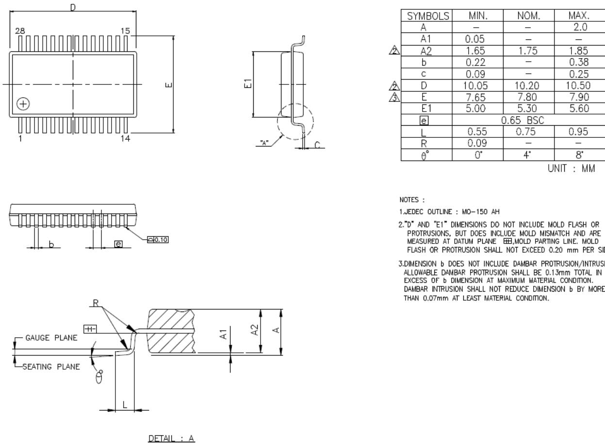
Figure 9.1 SSOP-24 Package Dimensions
