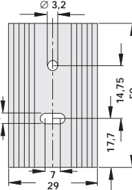
SK 09 50 TO 220
