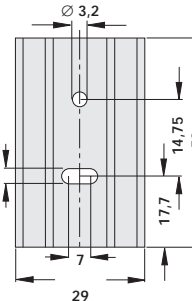
SK 145 50 TO 220
