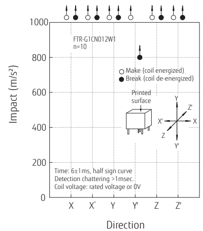
Shock resistance
