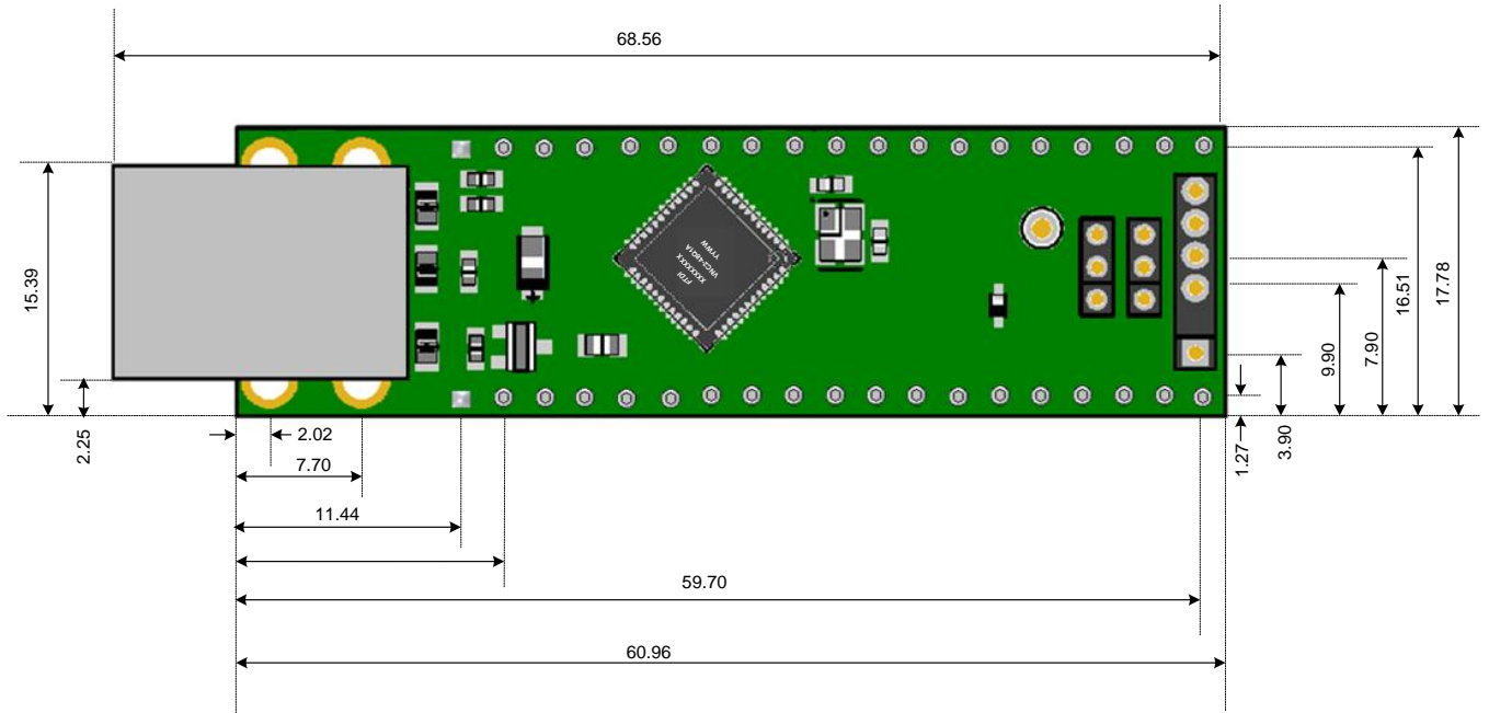
Figure 5.1 V2DIP2 48 Dimensions (Top View)
