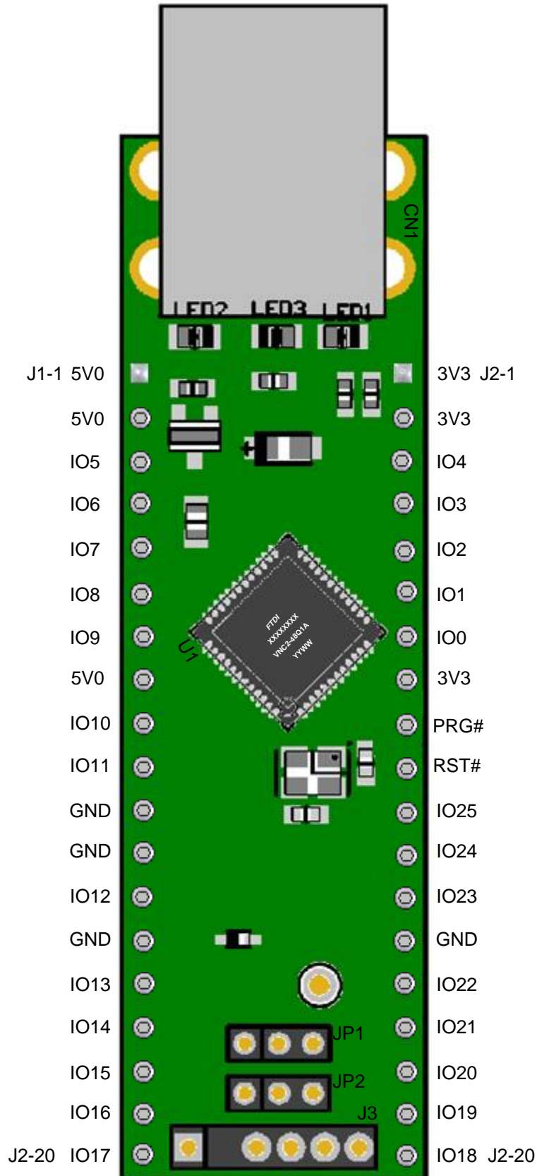
Figure 3.1 - V2DIP2 48 Module Pin Out (Top View)
